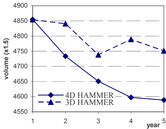
Average Hippocampal Volumes of 9 Subjects
