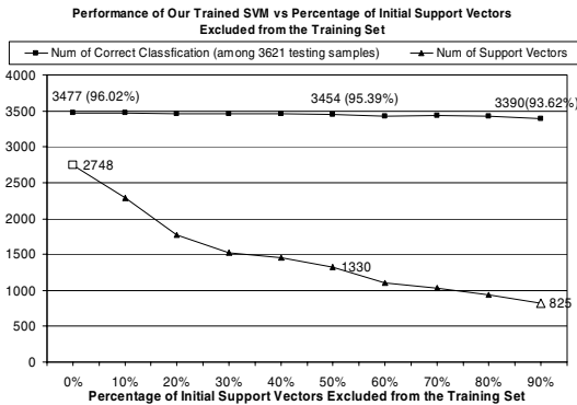
Fig. 3. (a) The performance of the finally-trained SVM changes with the percentages of initial SVs excluded from the training set. (b1-b2) Comparisons of tissue classification results using (b1) the original SVM with 2748 SVs and (b2) our trained SVM with 825 SVs. The tissue classification results are shown only in an ellipsoidal region
